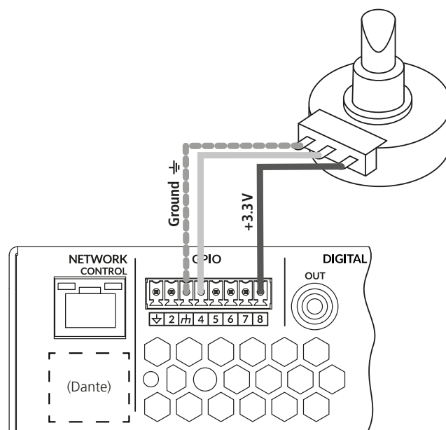
Fig. 10 external volume control
