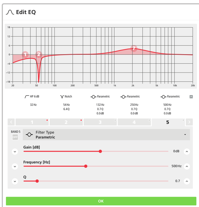
Fig. 27 Window "Output – Edit Equalizer"
