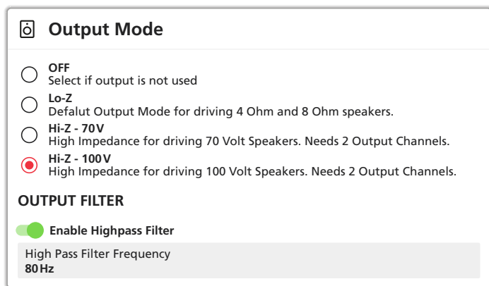
Fig. 32 View “Output – Speaker Preset – Output Mode”
