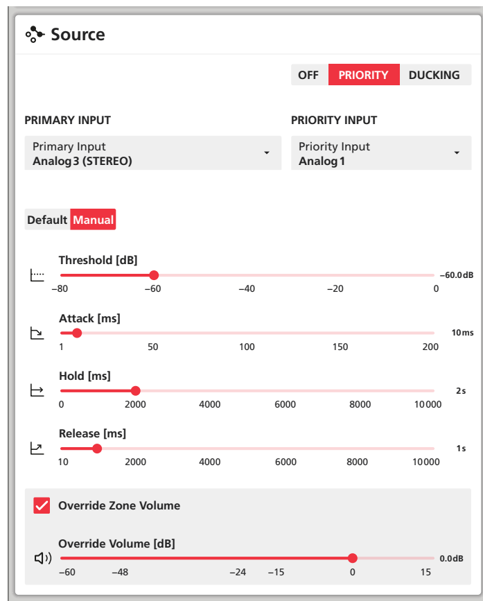
Fig. 20 View "Zone – Source"
