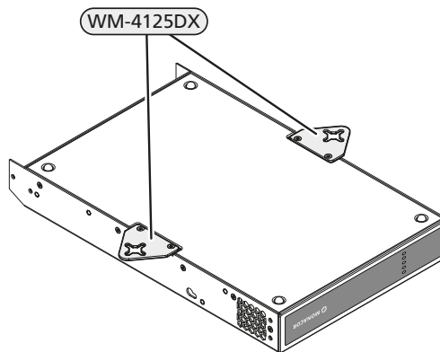
Fig. 8 Mounting plates on lower side of the device
