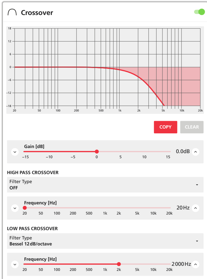
Fig. 30 View "Output – Speaker Preset – Crossover"
