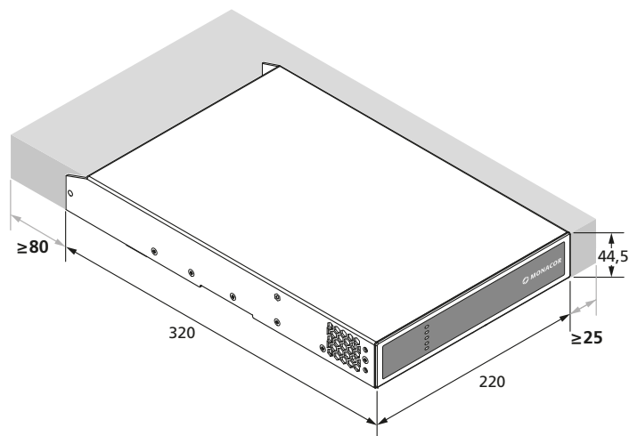
Fig. 4 Ventilation distances
