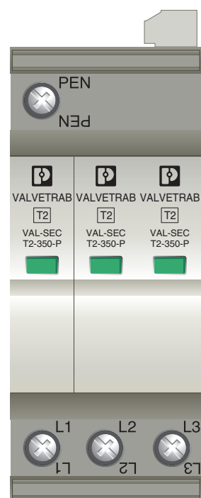
Product drawing
