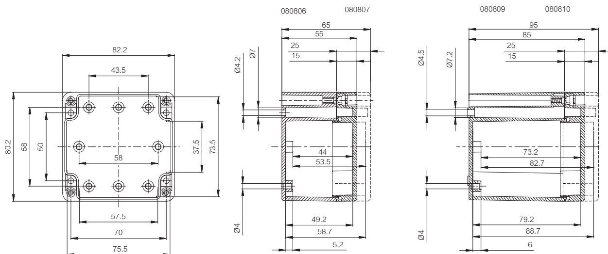
EURONORD PC/ABS 82x80x55-95
