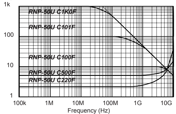
Impedance (ohm)
