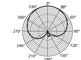
9 Diagrama polar vertical
