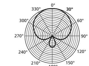
8 Diagrama polar horizontal
